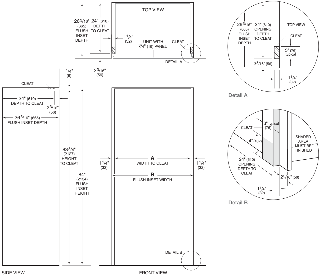
SIDE VIEW
